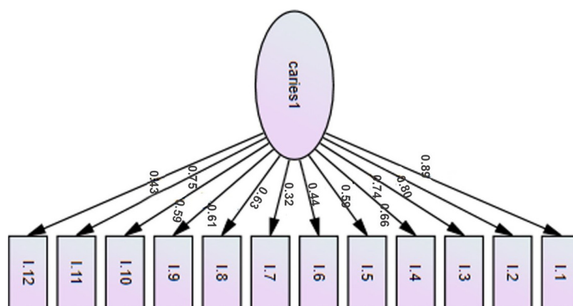
Figure 1. Standardized factor load, one-factor CFA model
